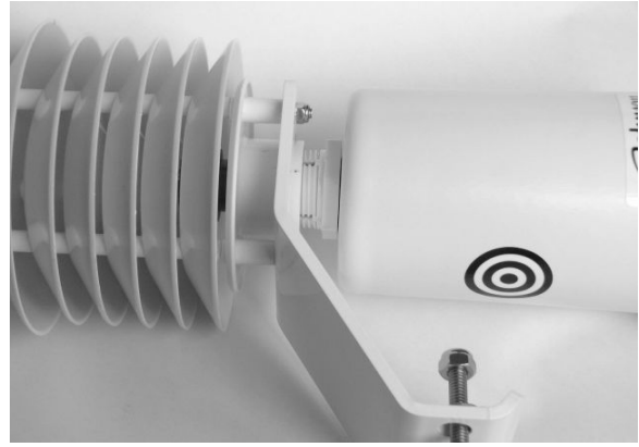
3. Hand tighten nut into shield
